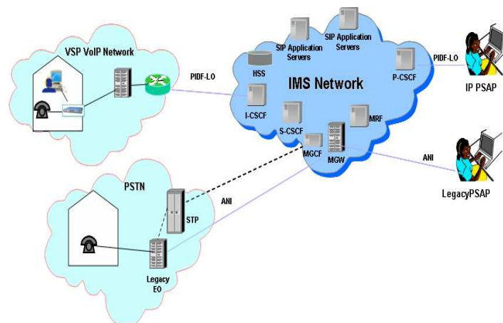
Figure 2 - Emergency Call Delivery from VoIP Towards Legacy PSAP
