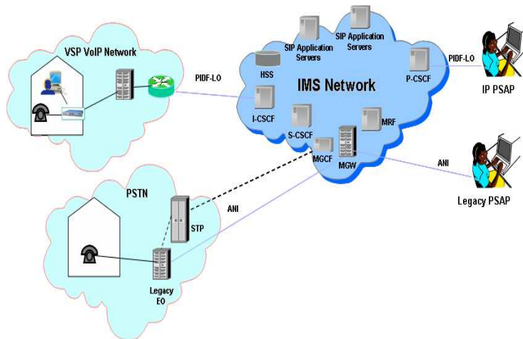
Figure 3 - Emergency Call from Legacy PSTN to IP PSAP
